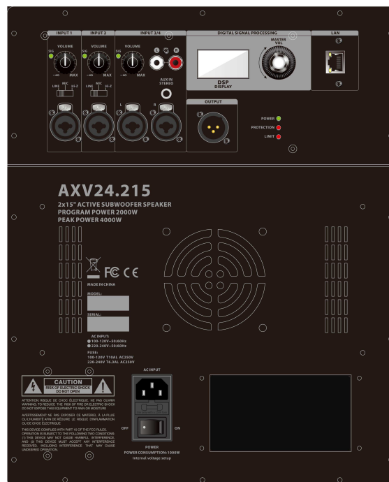
Subwoofer Back Panel
